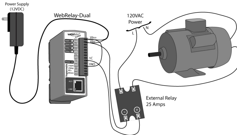
Figure 2.2d—External Relay Connection
