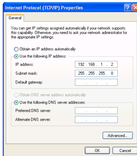
Figure 2.3f—TCP/IP Properties
