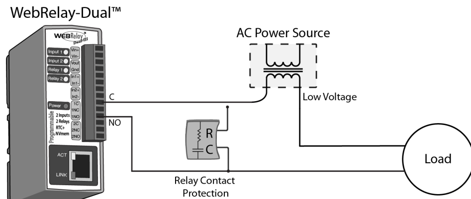
Figure 2.2f—AC Contact Protection
