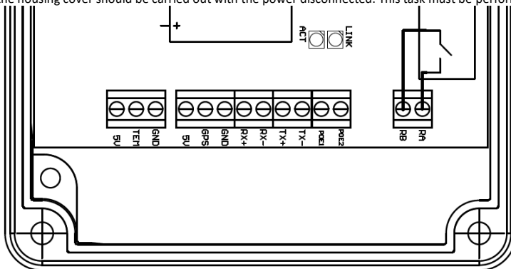
Fig. 1. Prestige Line clock connectors
