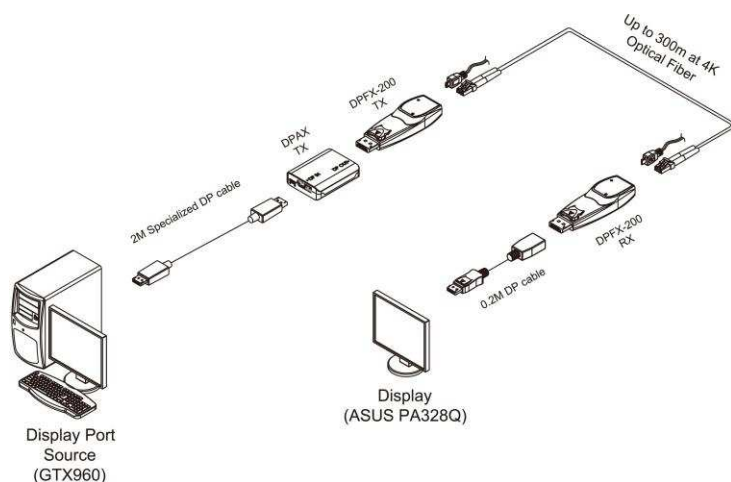
Figure 6- Connection of DPFX-200 and DPAX
