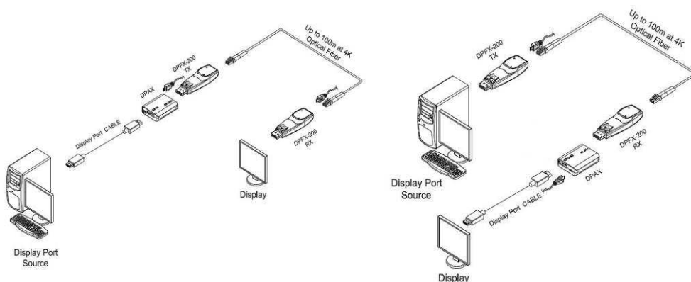
Figure 5 – Connection of DPFX-200 and DPAX (TX & RX)
