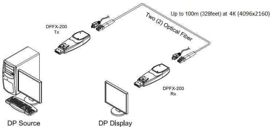
Figure 1 – Overall Connection of DPFX-200-TR
