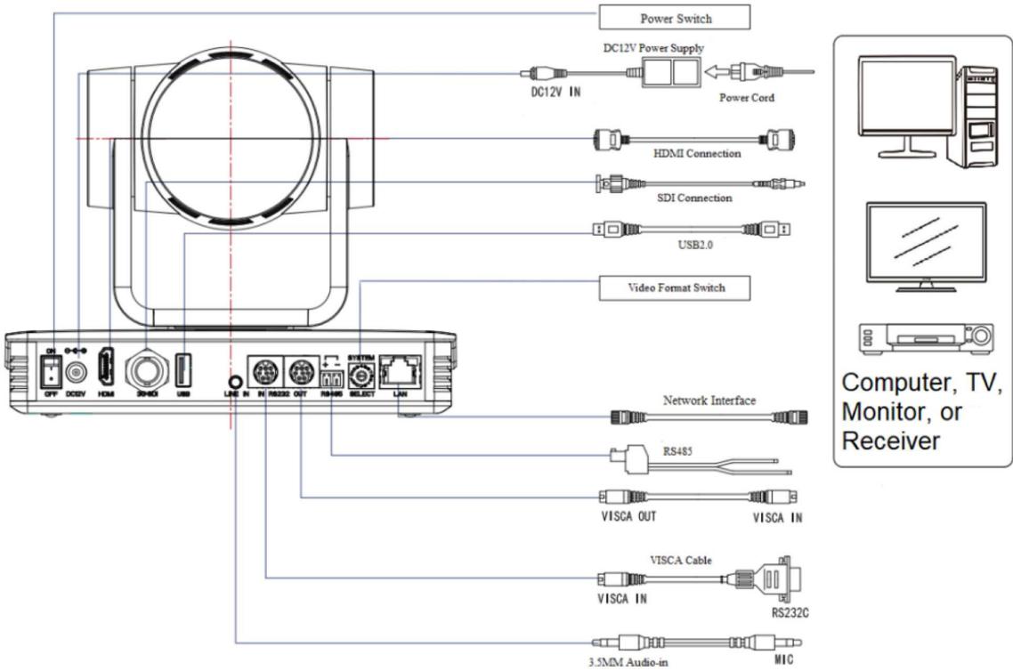
Wiring Diagram
