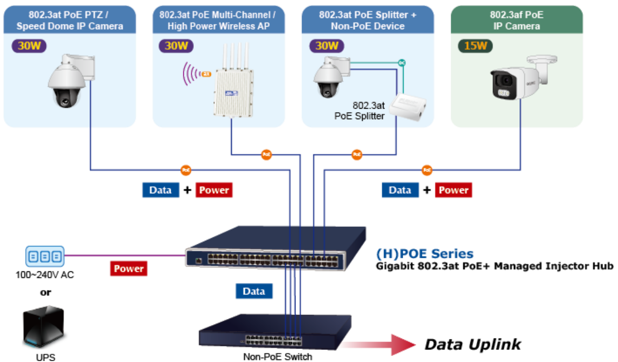
Figure 2-2-3: Network application installation
