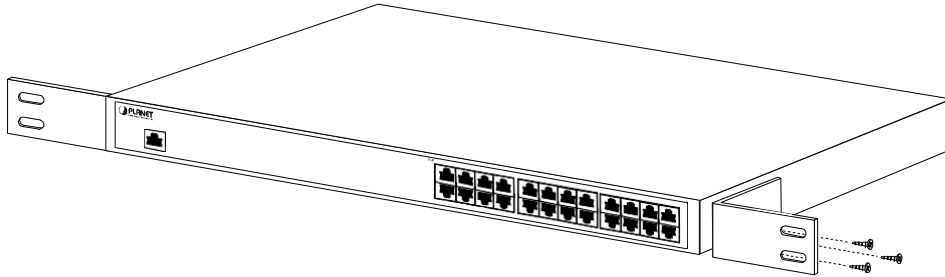
Figure 2-2-1: Brackets attaching to the PoE+ Managed Injector Hub
