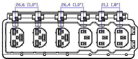
VIEW B
