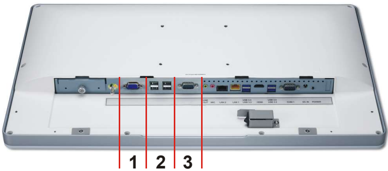
I/O Sections
