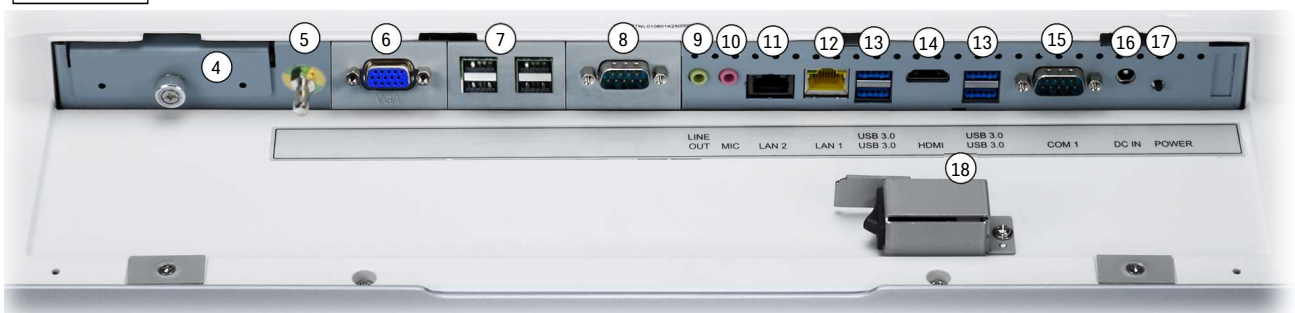
Back Panel
