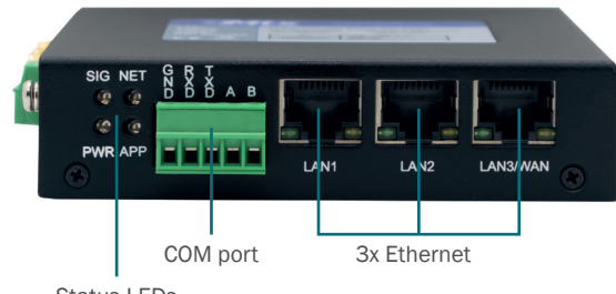
Status LEDs
