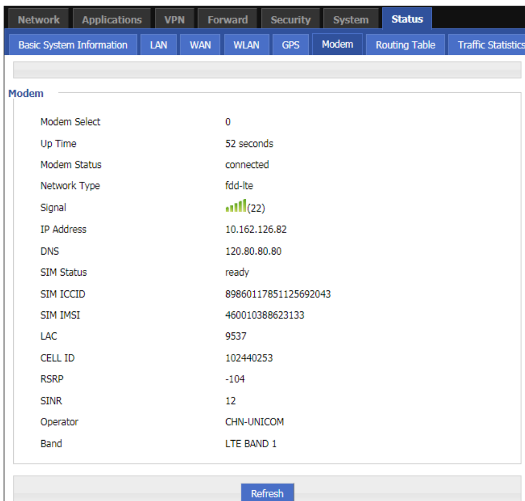
Figure 5-84 The page of Modem Status
