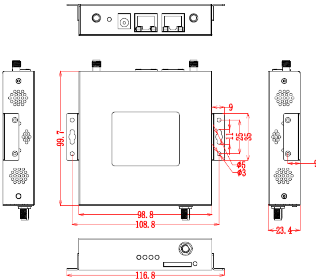
Figure 2-2 H8951 4G router views
