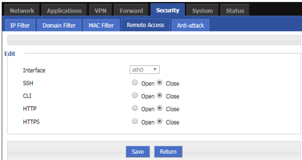
Figure 5-34 The editing page to open Ports
