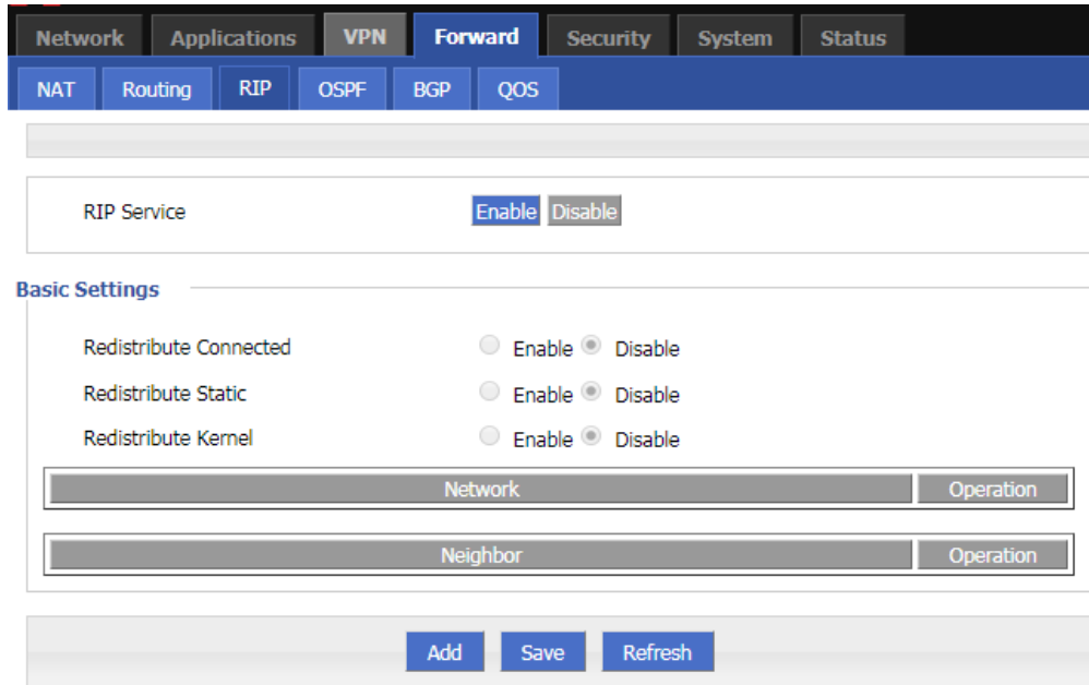
Figure 5-47 The configuration of RIP
