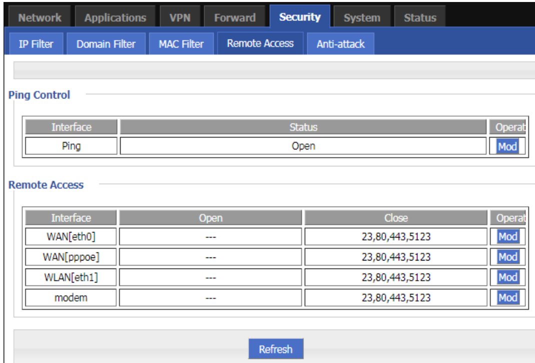
Figure 5-33 The page of "Remote Access"
