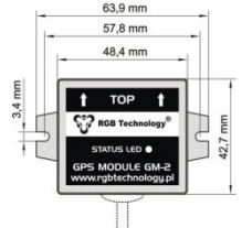
Fig. 1. Receiver module GPS GM-2 – overall view
