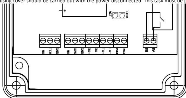
Fig. 1. Prestige Line clock connectors
