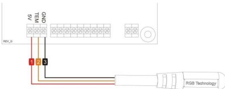
Fig. 4 Temperature probe and CC Extender wiring diagram
