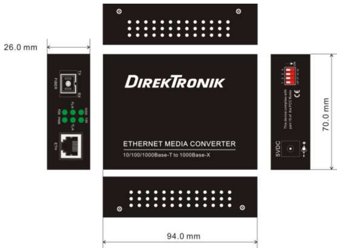
Mechanical Dimensions ( For external power adaptor type)
