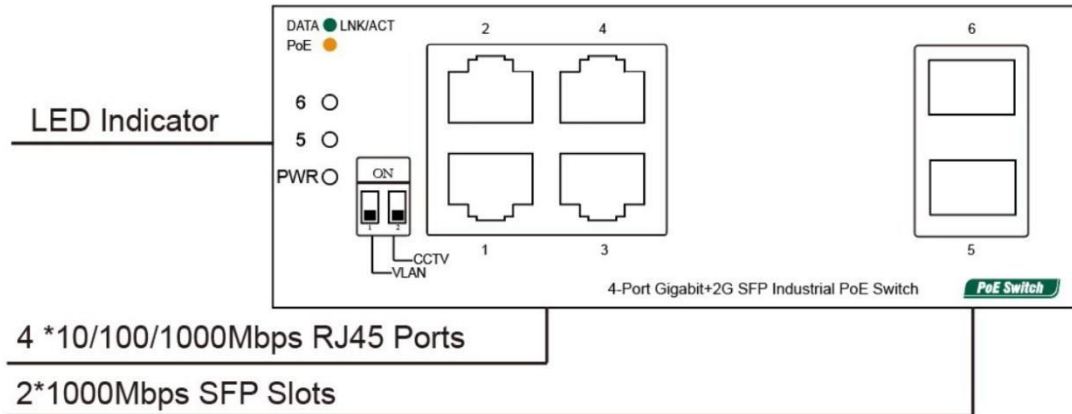
Figure 3-1 Front panel of 20117398
