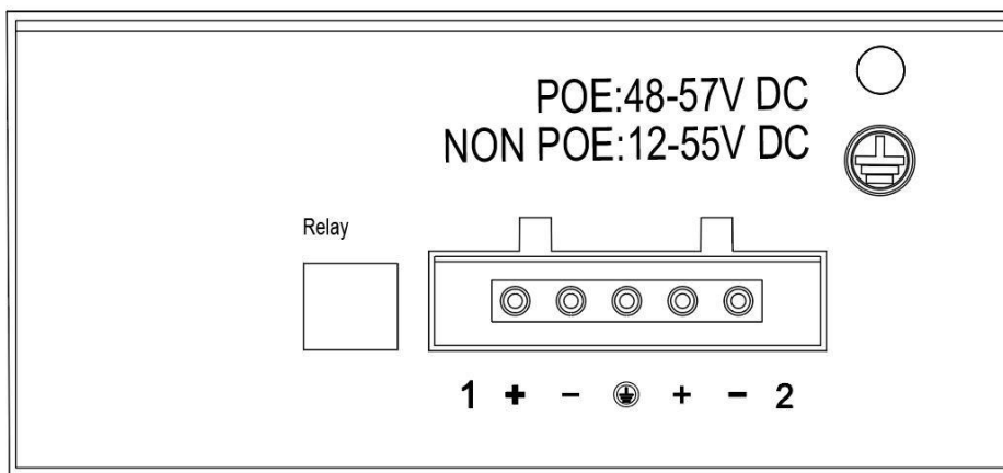
Figure 3-2 20117398 Switch side panel
